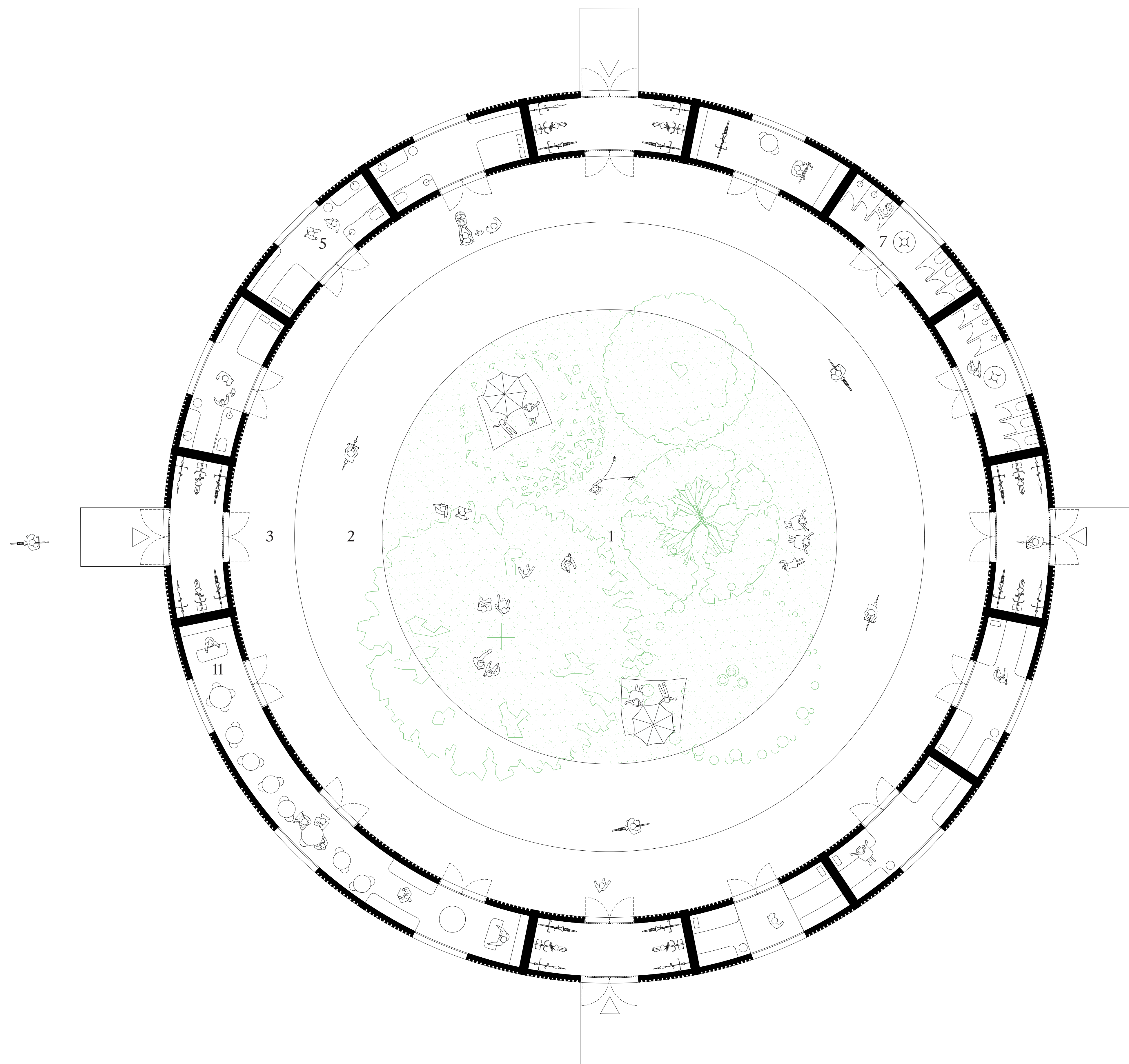
Ground level plan of the complex
